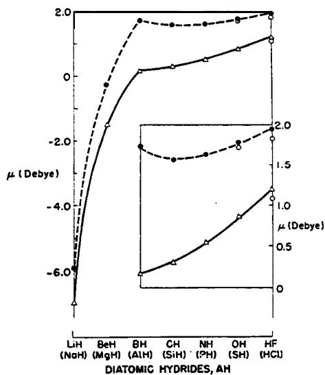
Fig. 10. The dipole moment for the ground state of the first- and second-row hydrides; first-row calculated values (●), second-row calculated values (A), and experimental values (o). Right-hand scale for small inset figure and left-hand scale for large figure. Reproduced by permission of the authors 14 and of the American Institute of Physics.
