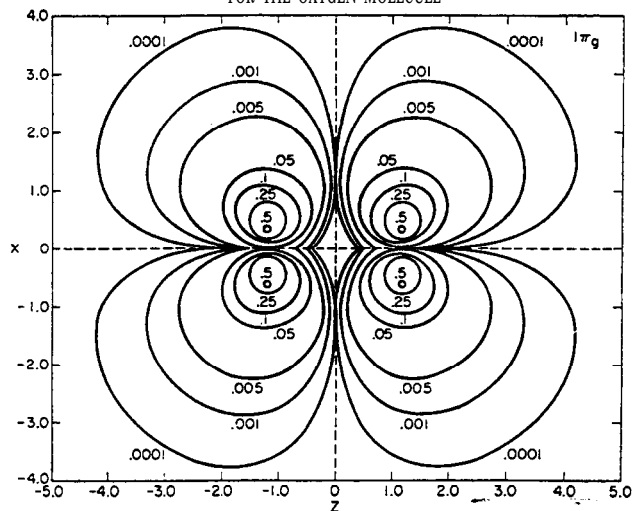
Figs. 1-5. Portraits of valence-shell spectroscopic MO's of the oxygen molecule. Each contour is marked with a number which is the square of the value of the MO on that contour. Each dashed line or curve marks a boundary between positive and negative regions of the MO itself. From an as yet unpublished paper by P.E. Cade, G.L.Malli and A. C. Wahl; all rights reserved.
