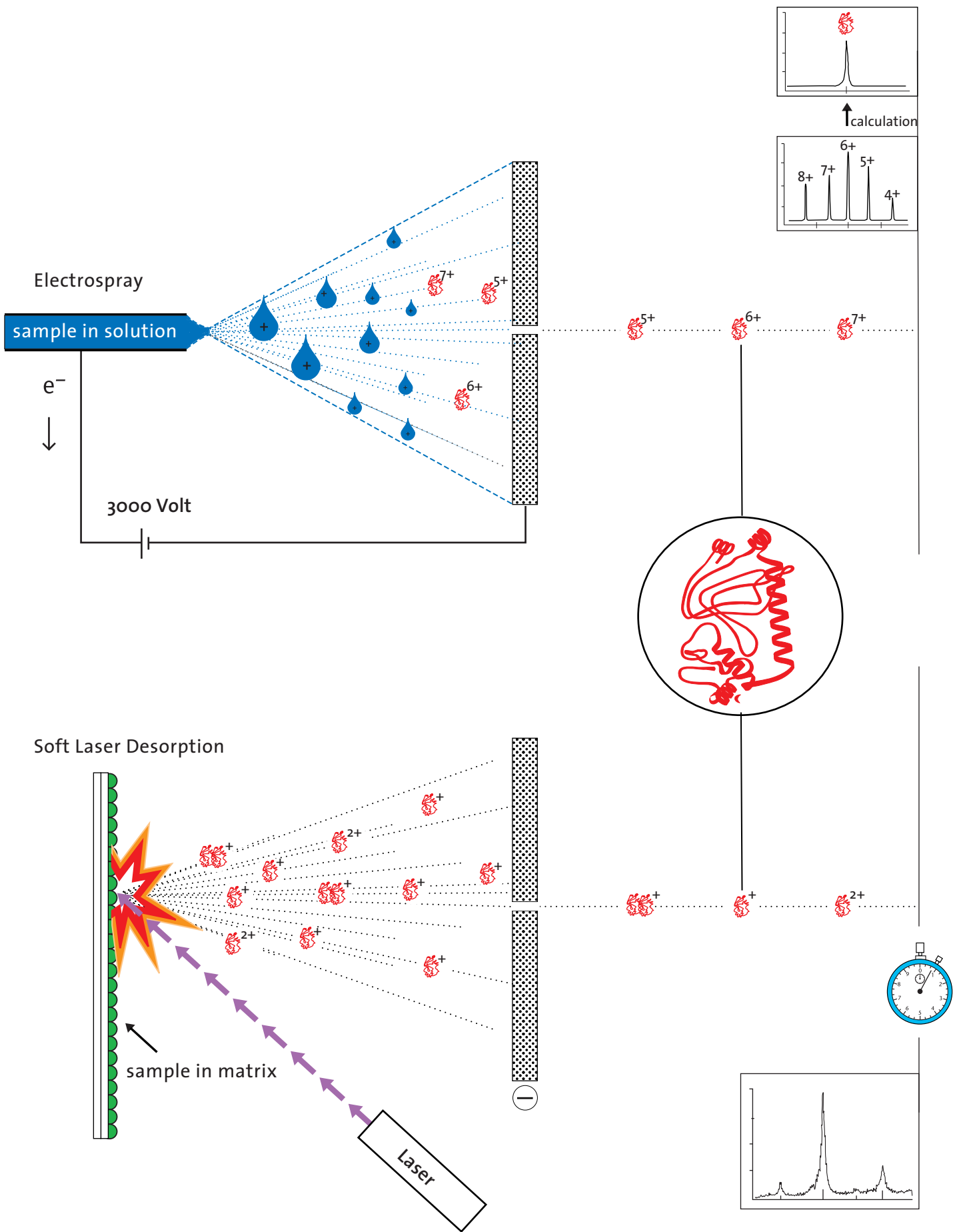
Fig 2. The principles for mass spectrometry of biomolecules. In ESI biomolecules are released as multicharged ions from small charged droplets. By ionisation with SLD (Soft Laser Desorption) the energy from the laser light is transferred to the biomolecules so that they enter the gas phase.
