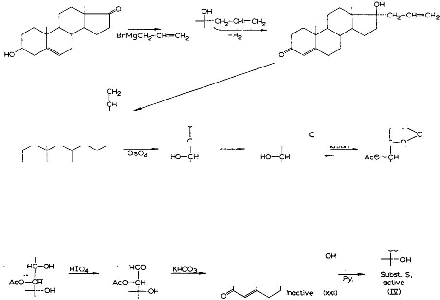
Scheme 6. Partial synthesis of substance S.
